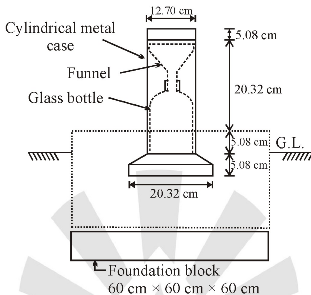
Fig. 2.1 : Symon's rain gauge
