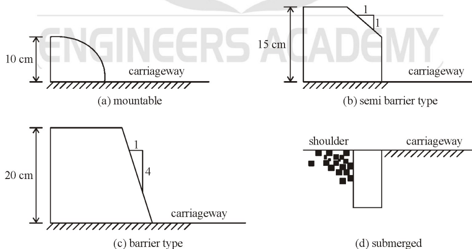
Fig. : Different types of kerbs
