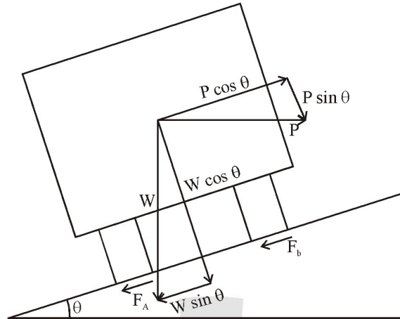
Fig. : Analysis of super-elevation
