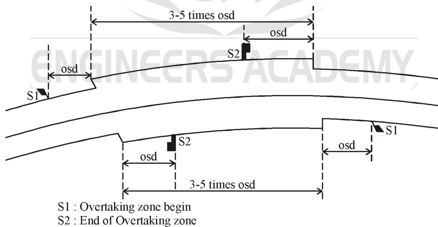
Fig. : Overtaking zones
