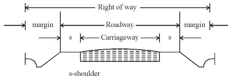
Fig. : Typical right of way (ROW)
