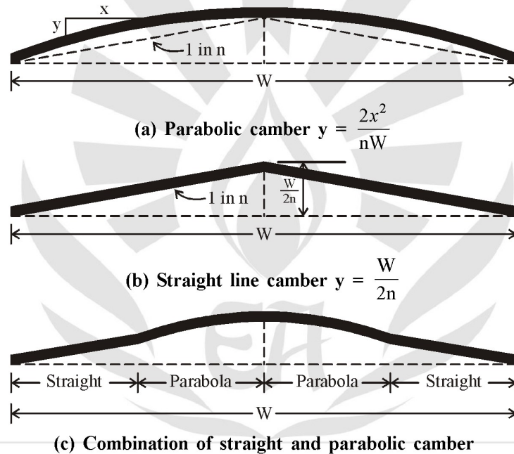
Fig. : Different types of camber
