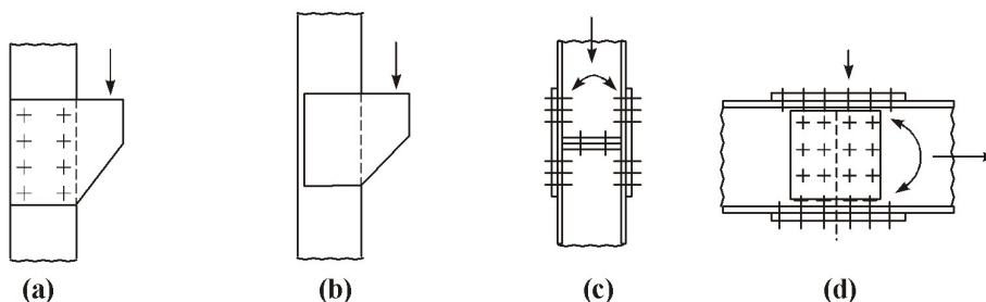
Example of 'rigid' connections (Martin and Purkiss 1992)
