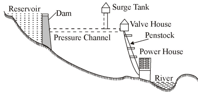
Schematic Arrangement of a Hydro-electric Plant
