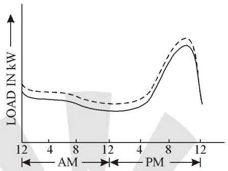
Typical Chronological Load Curve For Domestic Consumer
