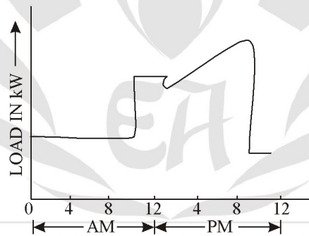
Typical Chronological Load Curve For Commercial Consumers
