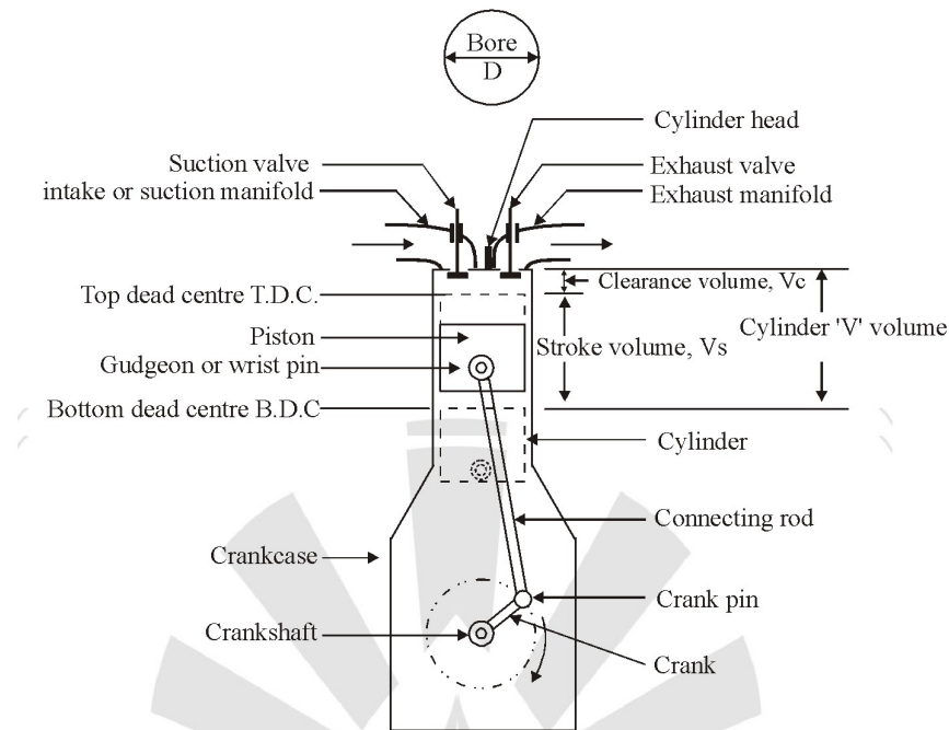
Fig. Important positions and volumes in reciprocating engine
