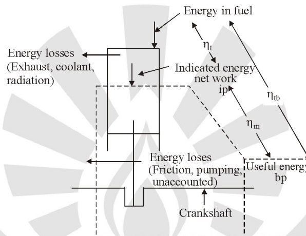
Fig. Energy flow through the reciprocating system
