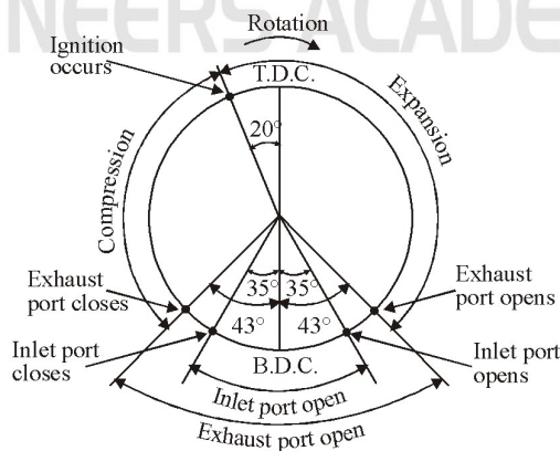
Fig. Typical valve timing of a two-stroke engine
