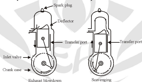
Fig. Crankcase-scavenged two-stroke engine.
