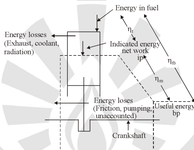
Fig. Energy flow through the reciprocating system
