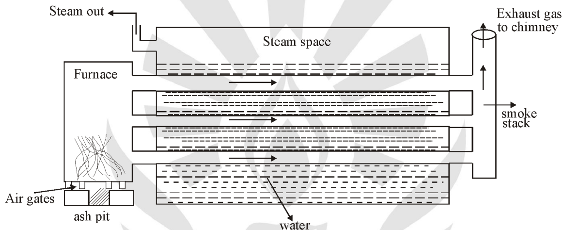
Fire Tube Boiler
