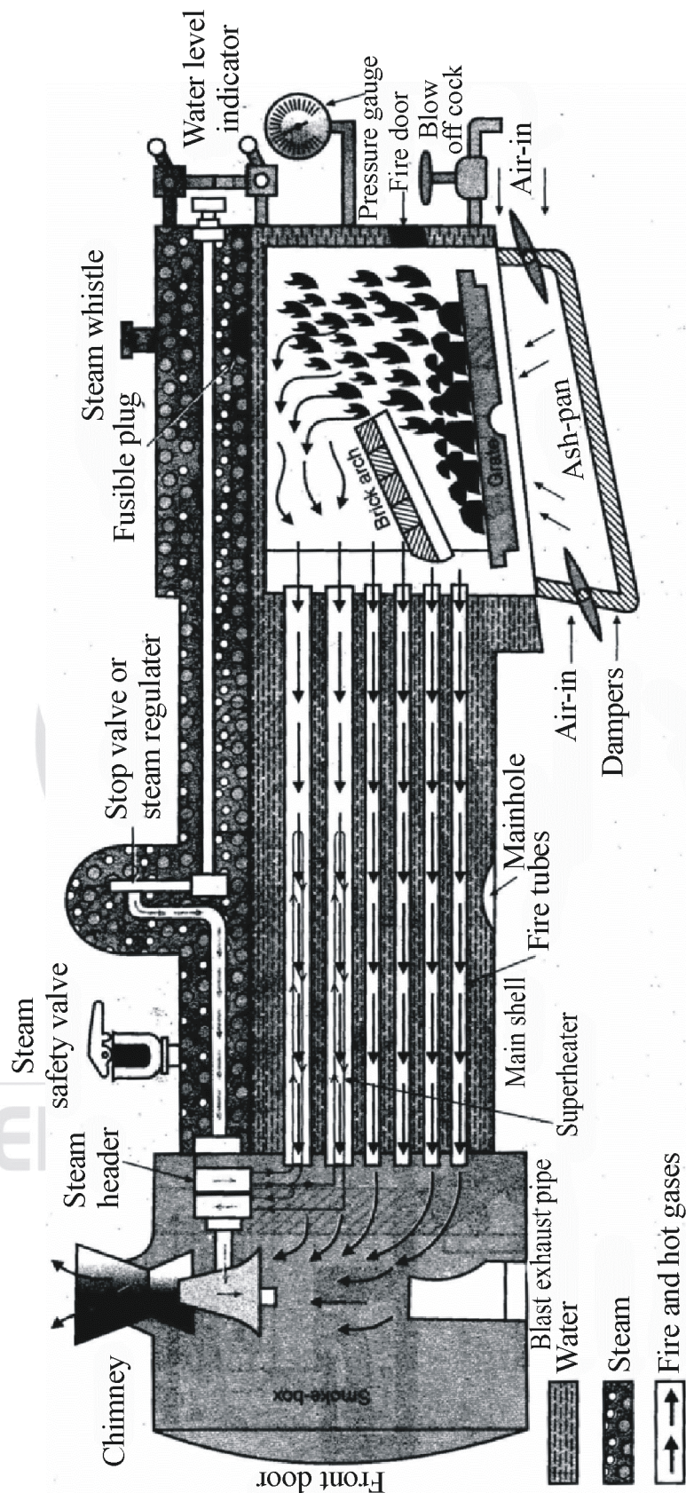
LOCOMOTIVE-BOILER
